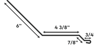
UNIVERSAL ENDWALL
