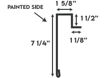
DOOR POST TRIM
