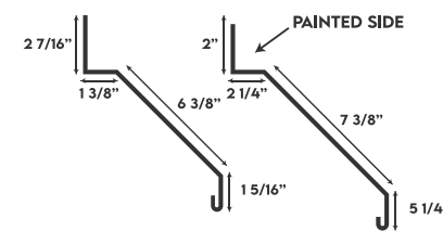
GABLE TRIM
