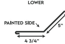
GAMBREL TRIM LOWER
