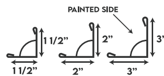
INSIDE ANGLE
