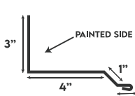
UNIVERSAL SIDEWALL
