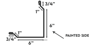
GABLE TRIM
