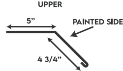
GAMBREL TRIM UPPER
