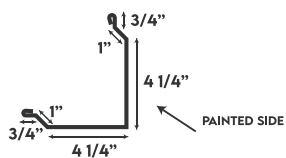
RAKE & CORNER
