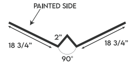
EXTENDED VALLEY
