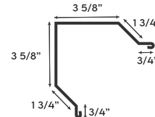
OUTSIDE CORNER
