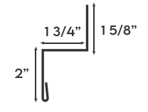
SIDEWALL TRIM
