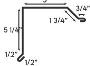
ECONOMY RAKE
