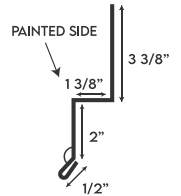
ZEE TRIM
