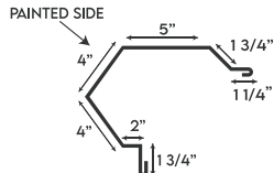
RAKE TRIM
